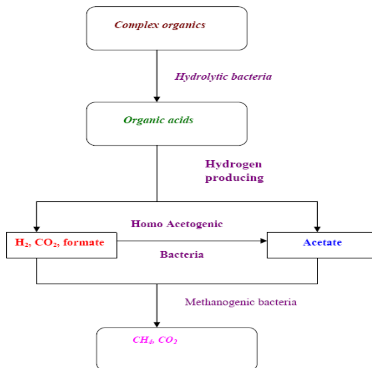
Figure 3: Biogas production process (Omer, 2003)
