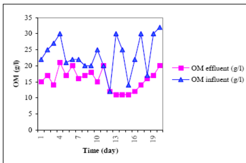
Figure 5: Organic matters before and after treatment in digester (Omer, 2006).
