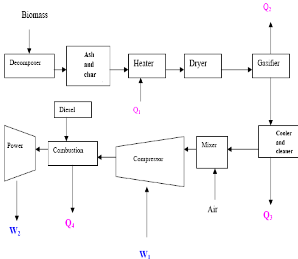
Figure 7: Advanced biomass power with diesel engine (Omer, 2006).
